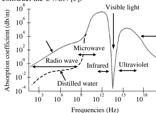
Figure 3. Absorption coefficients of electromagnetic wave in the water.
