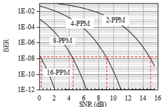
Figure 14. BER versus SNR for L -PPM with different L values.
