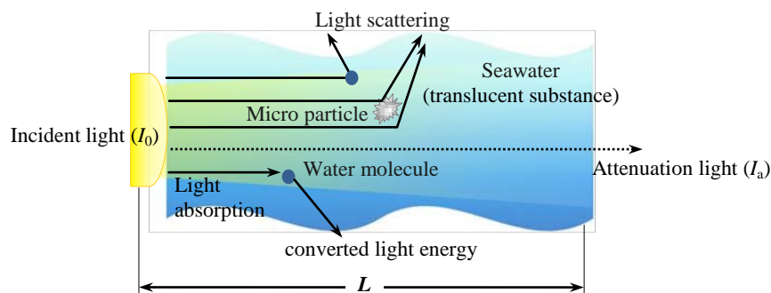
Figure 4. Physical model of light propagation in seawater.
