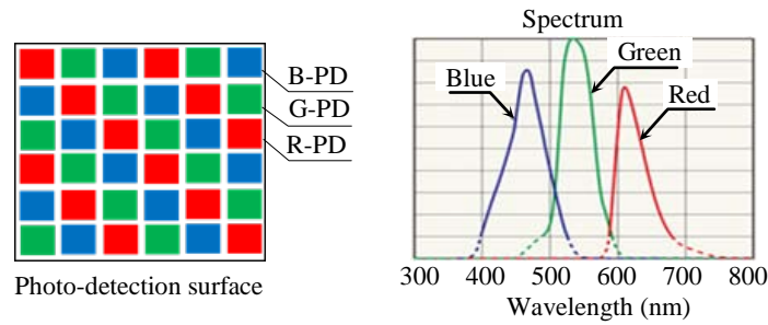
Figure 12. Three-sensors color photodiode.
