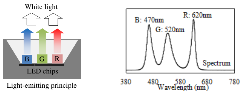
Figure 11. Three-chips white LED module.
