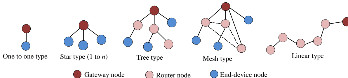
Figure 8. The link topologies of different UWSN type.
