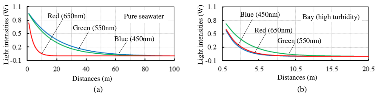
Figure 5. Spectrum-intensity attenuation for different seawater types in horizontal direction: (a) pure seawater and (b) bay.
