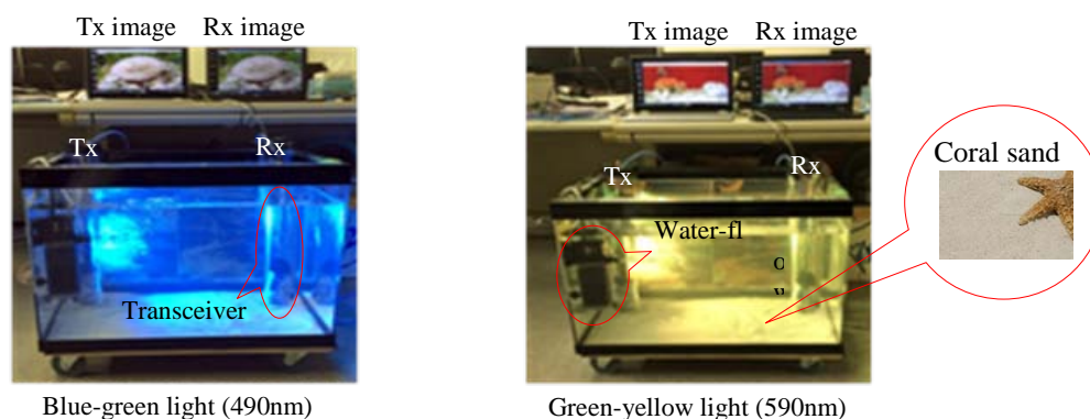
Figure 17. The results of underwater one-to-one image transmissions with different light wavelength.
