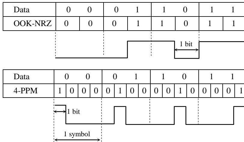
Figure 13. The coding methods of OOK-NRZ and 4-PPM.
