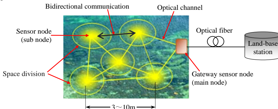
Figure 9. The mesh-type UOWSN.
