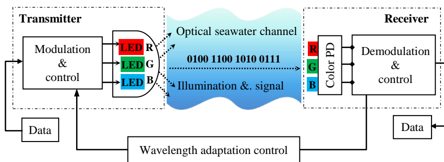
Figure 10. LED-based VLC transceiver with wavelength adaptation control.
