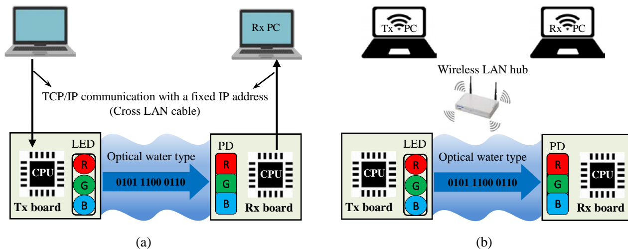
Figure 16. System work modes: (a) wired and (b) wireless mode.
