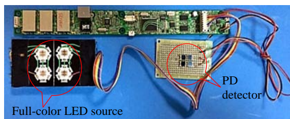
Figure 15. The prototype of LED-based VLC transceiver.
