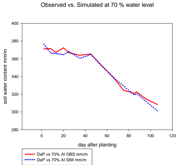
Figure 6. Observed Vs. Simulated at 70 % water level 2019 G.C.
