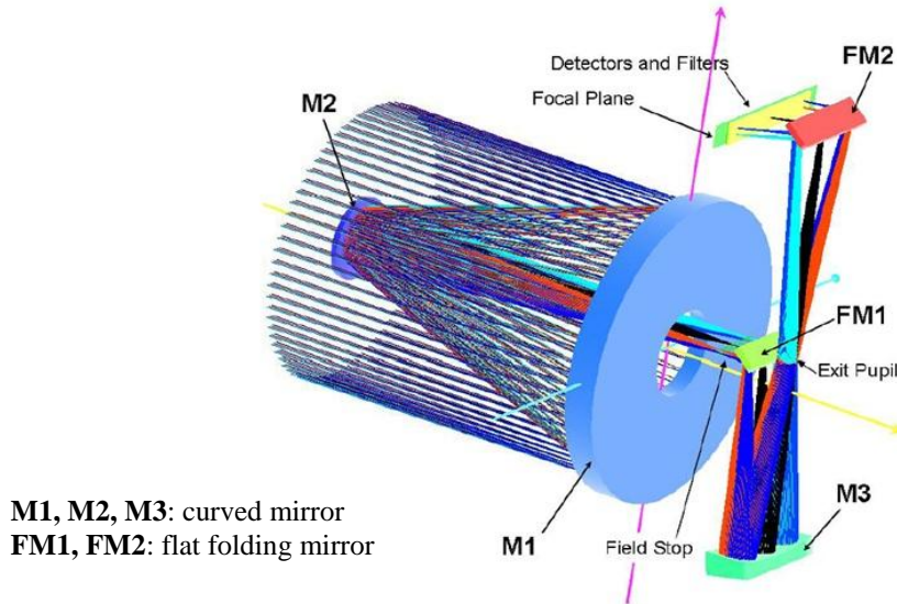
Figure 1. The optical concept of the Korsch telescope
