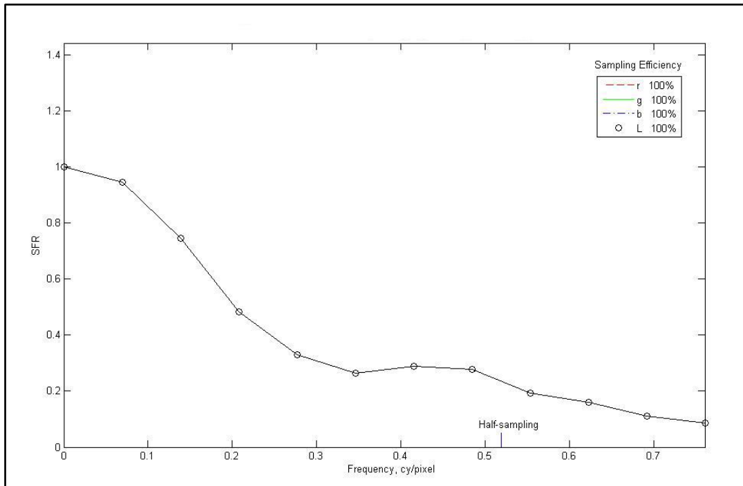
Figure 5. MTF@ Nyquist frequency in data taken on 25 th April 2016
