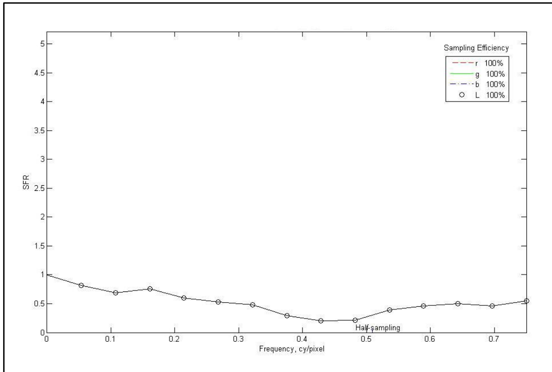
Figure 4. MTF@ Nyquist frequency in data taken on 18 th July 2016
