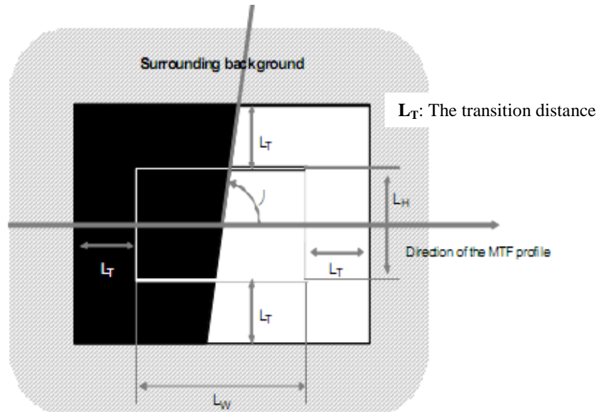
Figure 2. The design of edge target for MTF estimation
